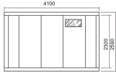
ALZADO PRINCIPAL
