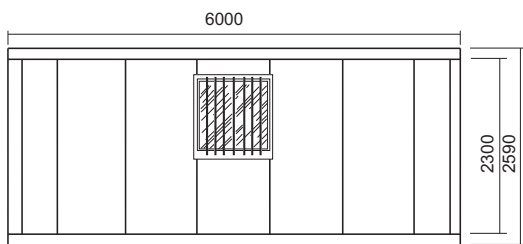
ALZADO PRINCIPAL
