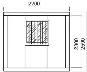
ALZADO PRINCIPAL
