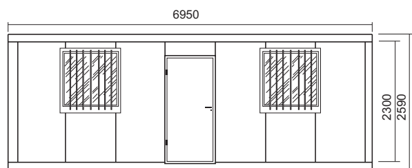
ALZADO PRINCIPAL
