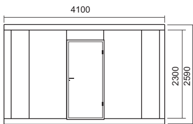
ALZADO PRINCIPAL
