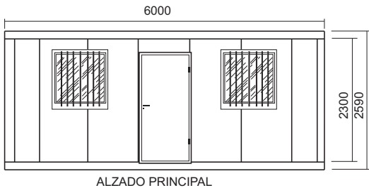
ALZADO PRINCIPAL
