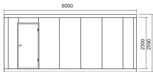
ALZADO PRINCIPAL
