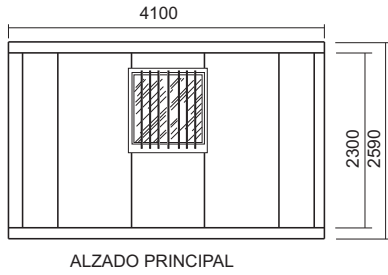
ALZADO PRINCIPAL
